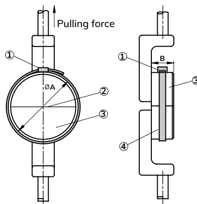
Figure2. Installation for parallel entry cable tie
