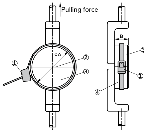
Figure1. Installation for standard cable tie
