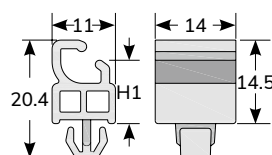
SWS-1 To fit hole
