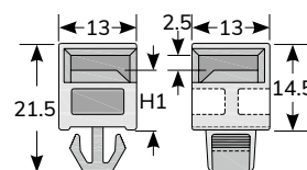
SWS-2 To fit hole
