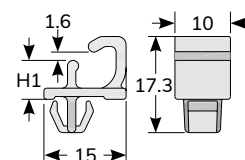
HGS-11 To fit hole
