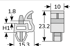
HGS-7 To fit hole
