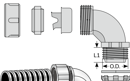
(Metal flexible conduit) RBG (control box adaptor)
