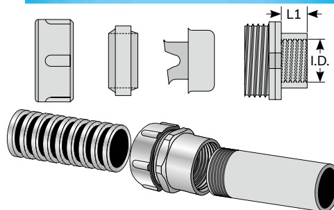
(Metal flexible conduit) FBG (PT thread for metal pipe)
