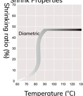
SUMITUBE C Shrink Properties
