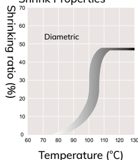
SUMITUBE A Shrink Properties
