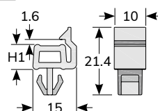
HGS-8 To fit hole
